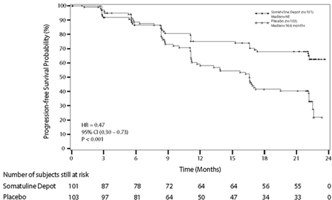
Figure 1: Kaplan-Meier Curves of Progression-Free Survival
